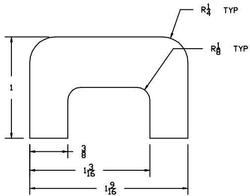
STANDARD ALNICO MAGNET USED IN TRADITIONAL SEISMOMETER DESIGNS
