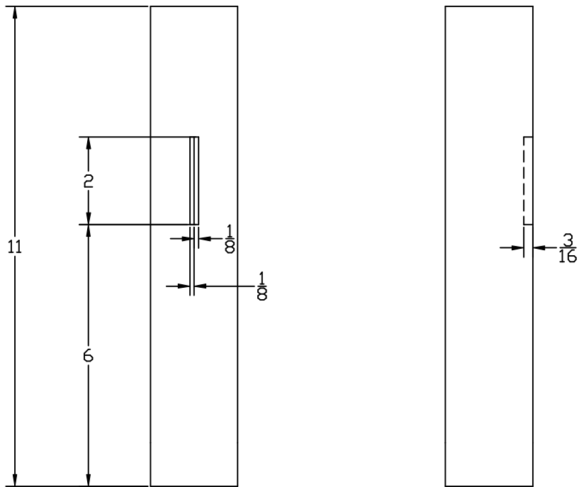
FRONT AND RIGHT VIEW OF SLOT FOR "KNIFE-EDGE"
