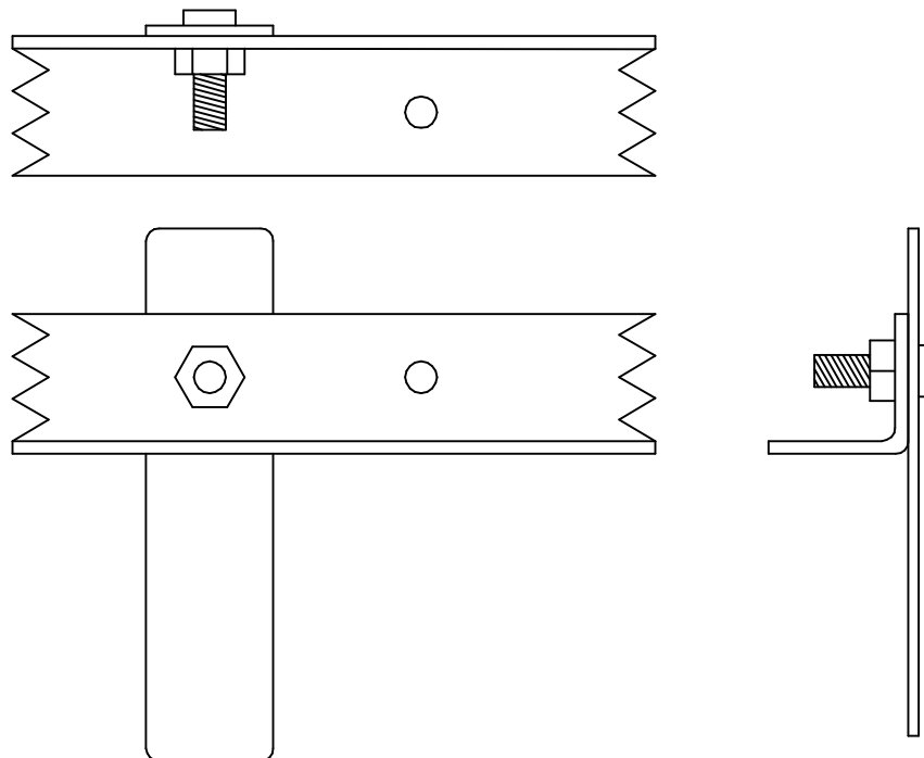
SECURING POINT FOR DAMPING PADDLE
